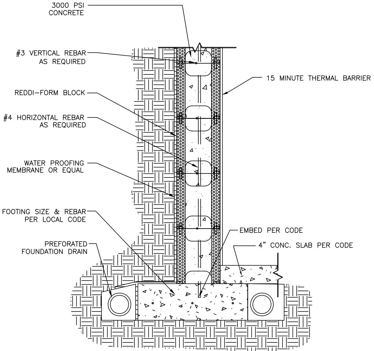
(F7) BASEMENT AND WALL FOOTING DETAIL 1" = 1'-0"
